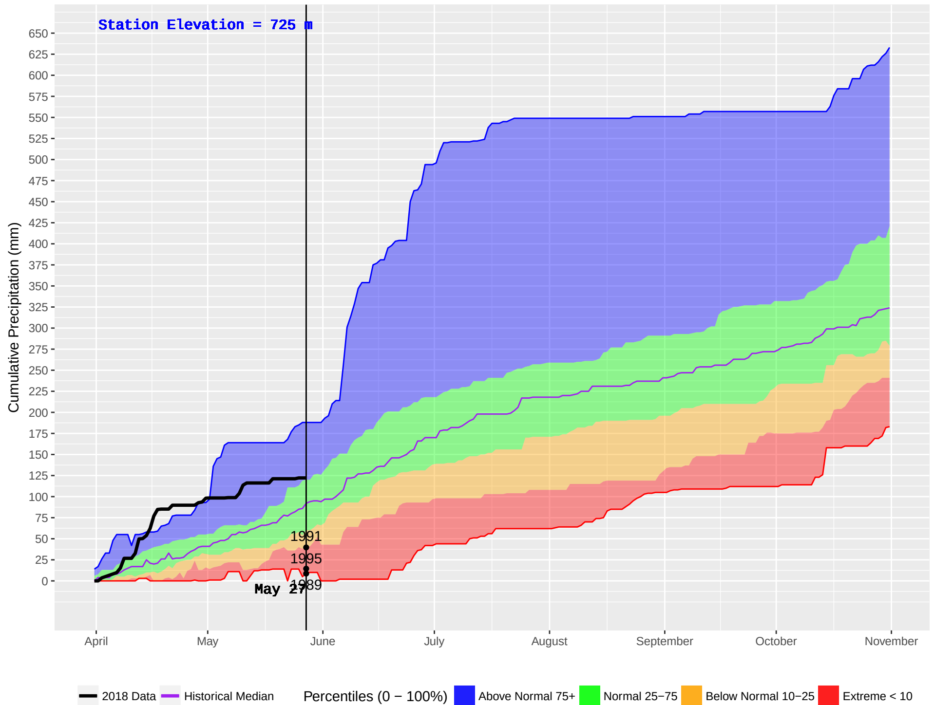
PENDOREILLE (402) : Historical (1986–2016) and Current (2018) Noon Cumulative Precipitation
