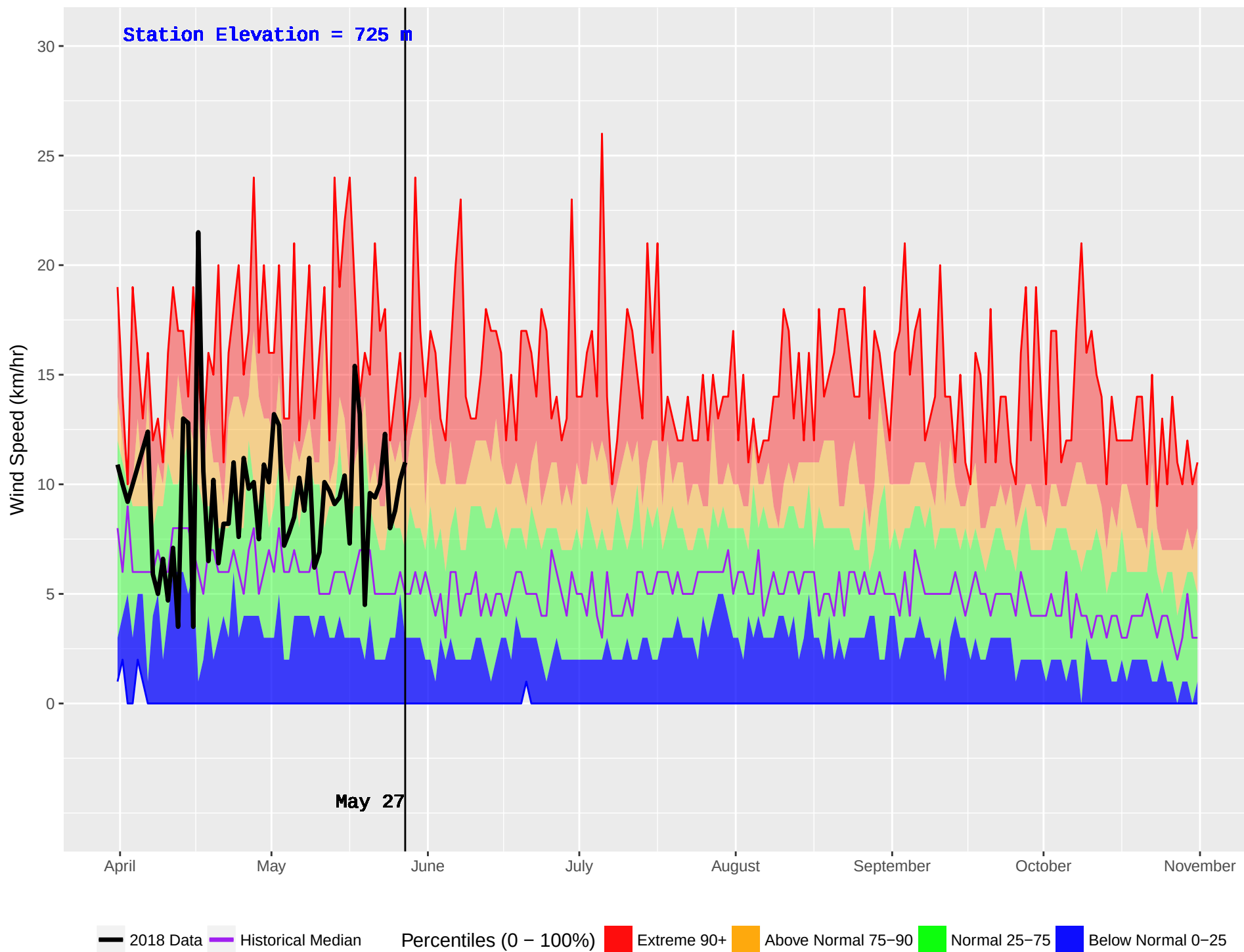
PENDOREILLE (402) : Historical (1986–2016) and Current (2018) Noon Wind Speed
