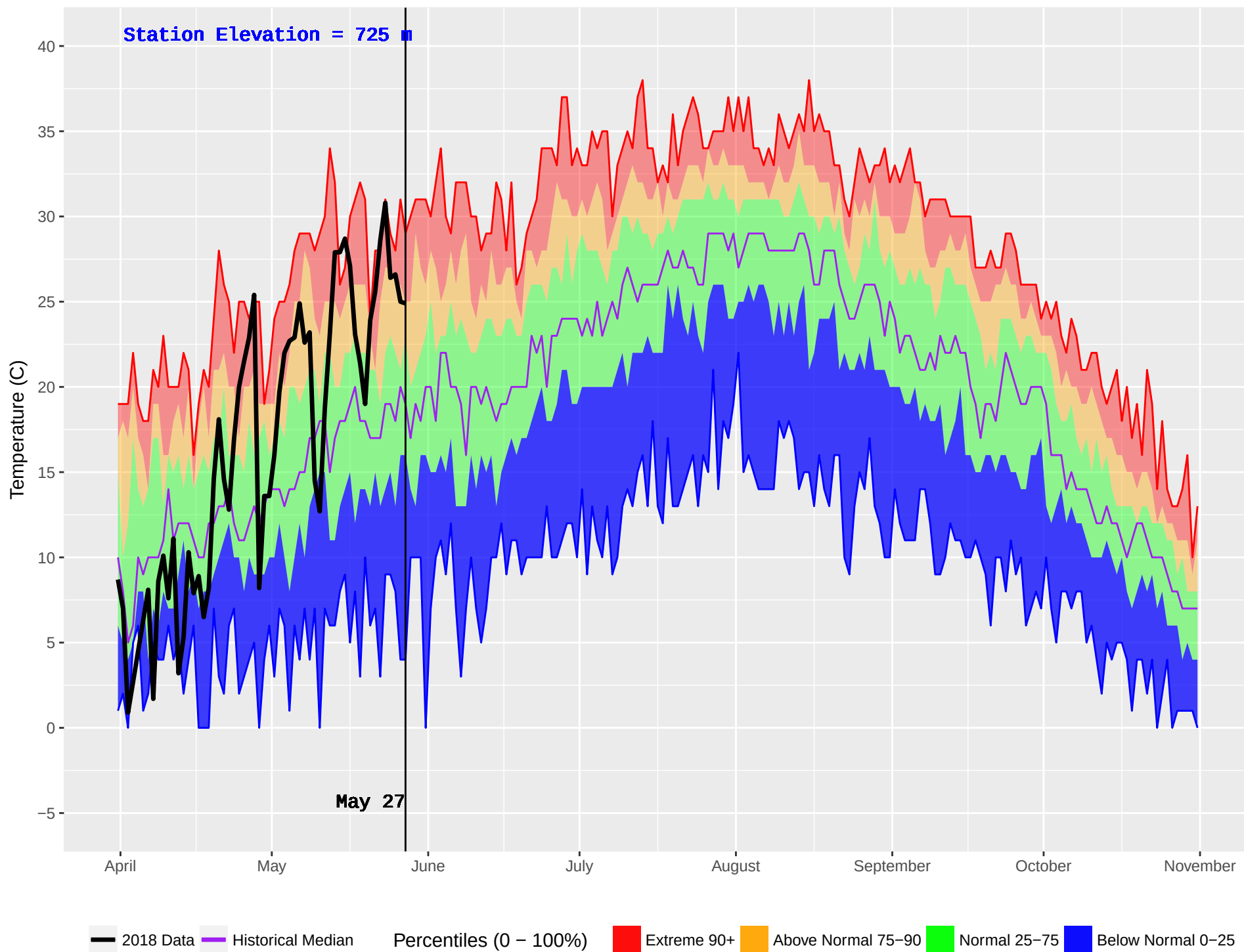
PENDOREILLE (402) : Historical (1986–2016) and Current (2018) Noon Temperature
