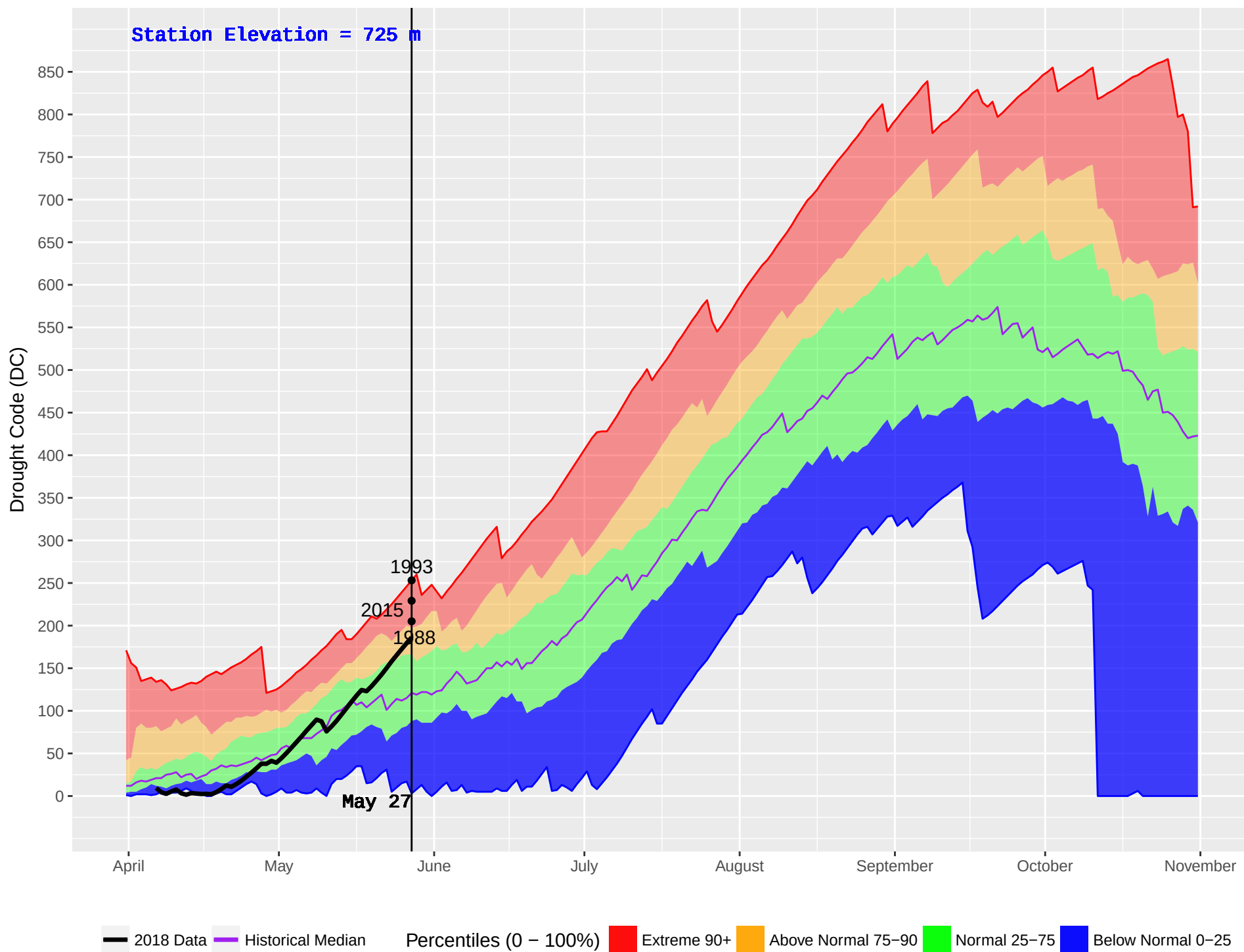
PENDOREILLE (402) : Historical (1986–2016) and Current (2018) Noon Drought Code (DC)
