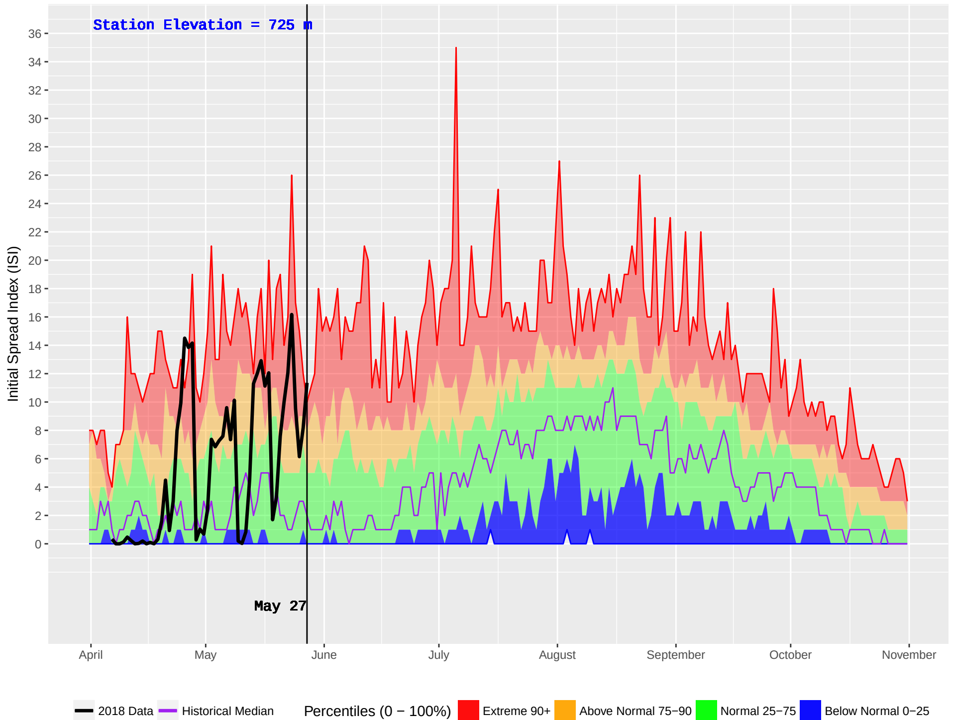
PENDOREILLE (402) : Historical (1986–2016) and Current (2018) Noon Initial Spread Index (ISI)
