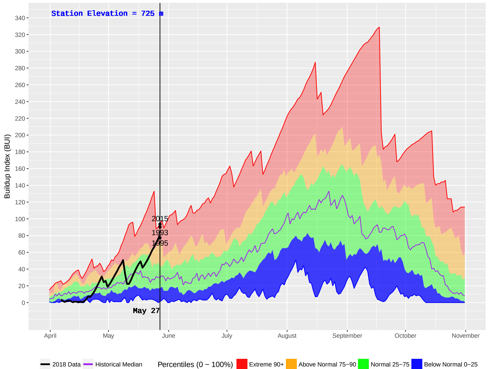
PENDOREILLE (402) : Historical (1986–2016) and Current (2018) Noon Buildup Index (BUI)
