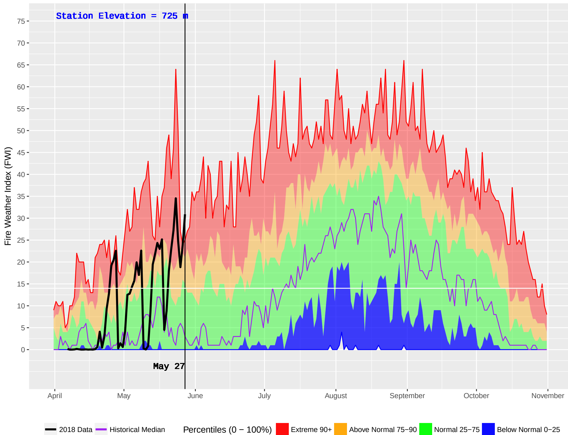
PENDOREILLE (402) : Historical (1986–2016) and Current (2018) Noon Fire Weather Index (FWI)
