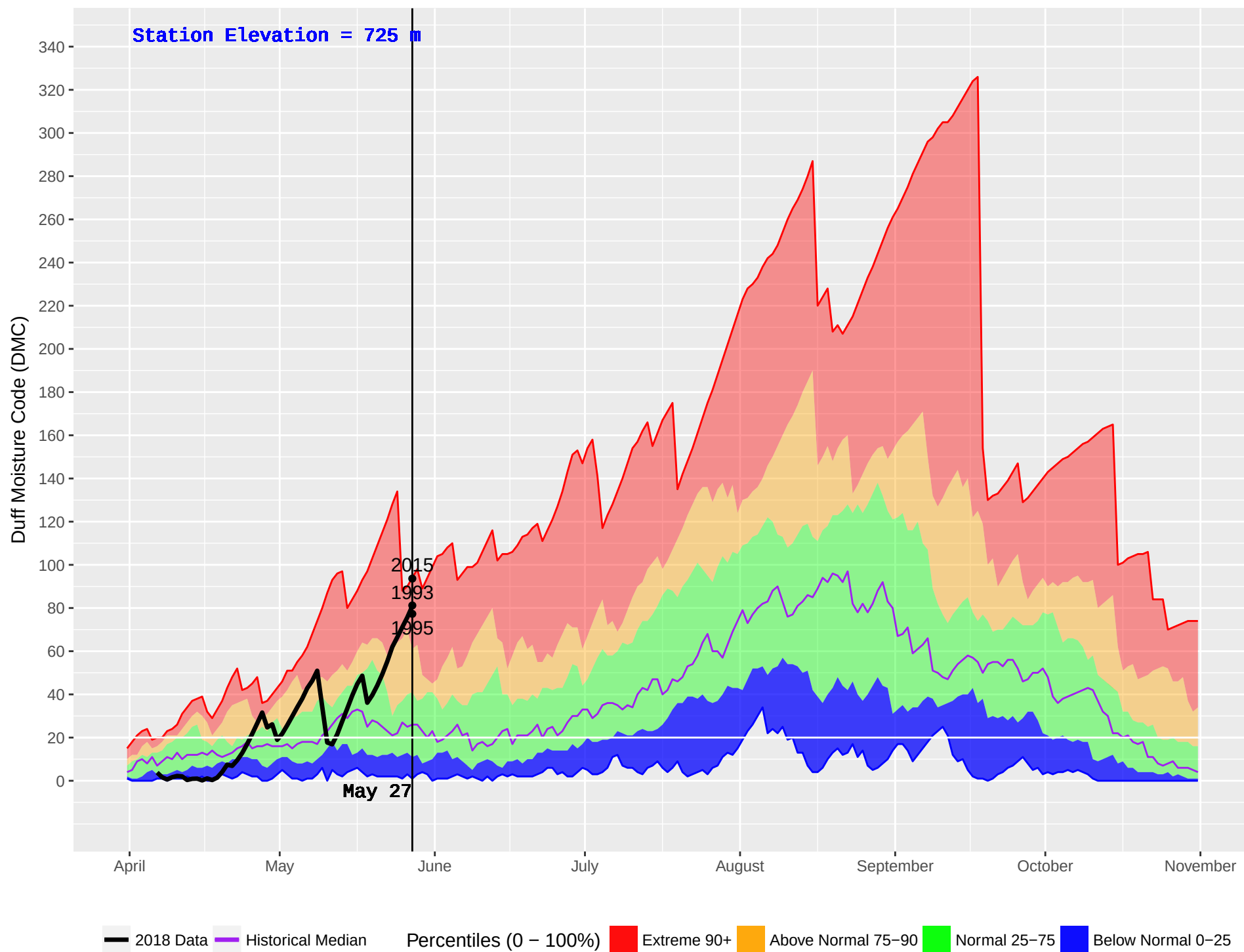
PENDOREILLE (402) : Historical (1986–2016) and Current (2018) Noon Duff Moisture Code (DMC)
